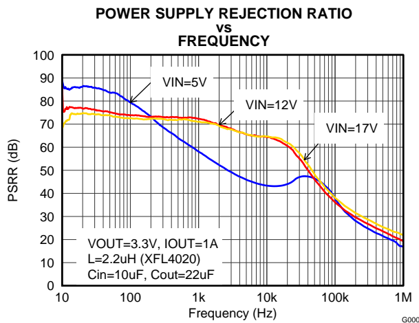
Figure 26. Power Supply Rejection Ratio, f_{SW}=2.5\text{MHz}
